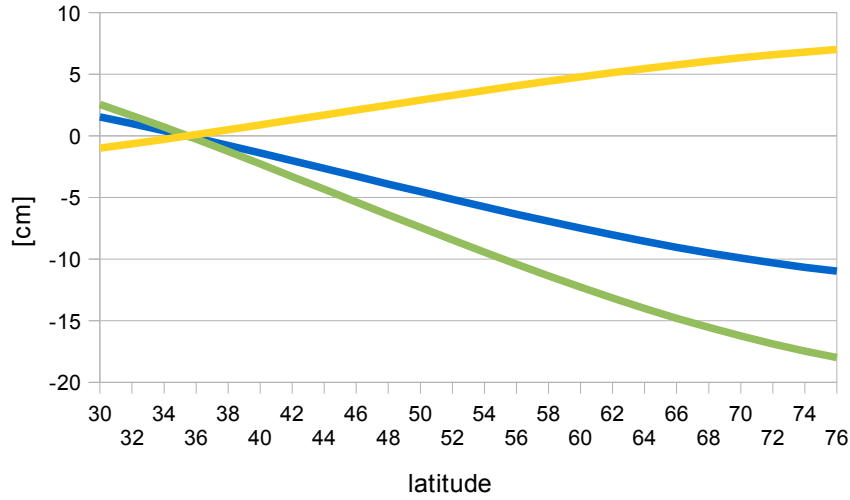
Fig.2 . Height changes over Europe caused by the application of different permanent tide concepts.
