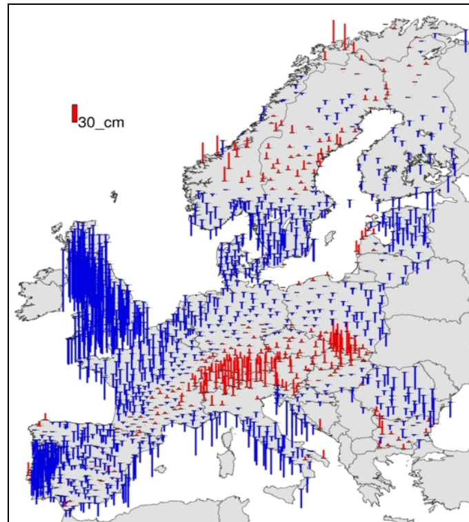
Figure 4. EUVN_DA and EGG97 height anomaly differences.
