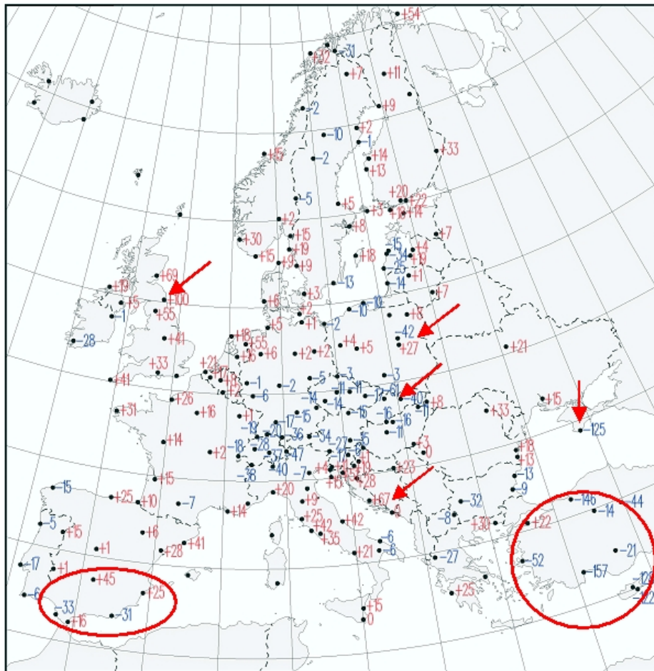
Figure.1 EGG97 and EUVN/UELN ( h^{\text{EUVN}} - H^{\text{UELN}} ) quasigeoid height differences [cm]. The original plot is taken from the EUVN final report, Ihde et al. (2000). The arrows and ellipses are indicating problematic points or areas.
